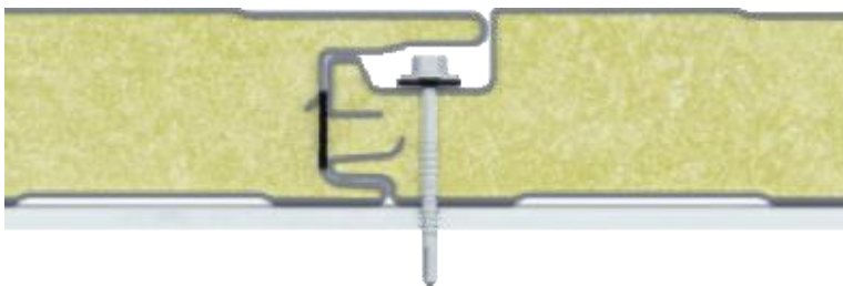
40 mm joint detail
